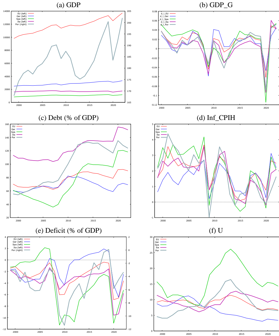
Figure 1: Macroeconomic Behavior (1999-2022)
